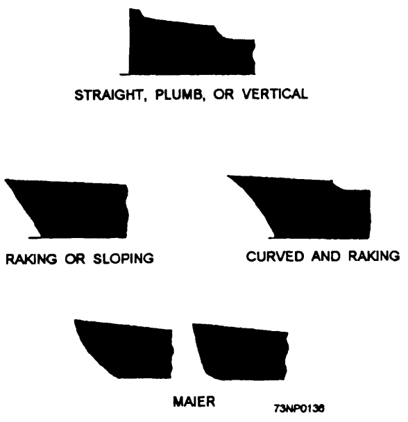
Figure 13-36.—Bow designs.
