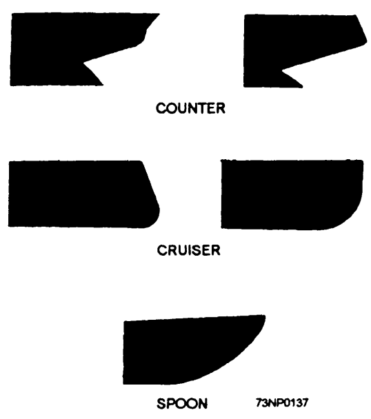
Figure 13-37.—Stern designs.
