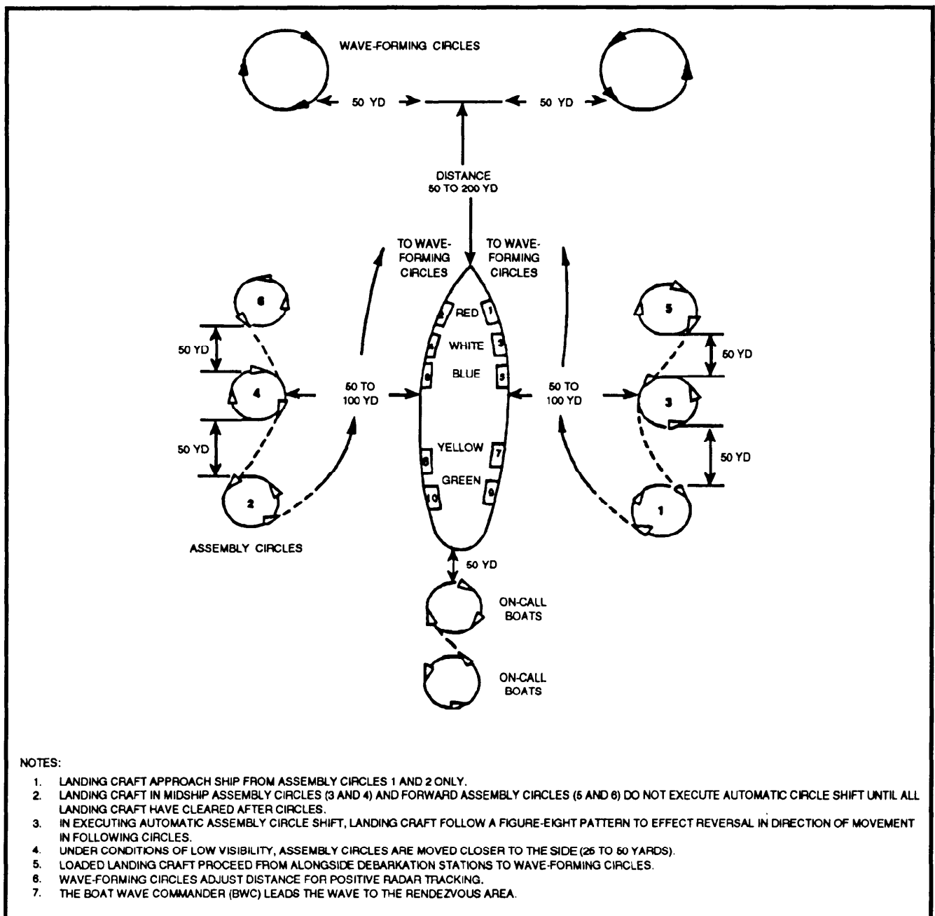
Figure 12-4.—Landing craft assembly circles.
