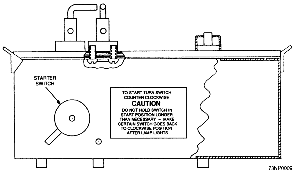
Figure 2-3.—Starter unit for 12-inch mercury-xenon searchlight.
