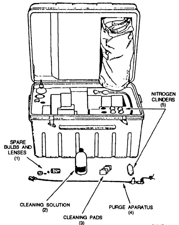
Figure 2-11.—Maintenance kit.
