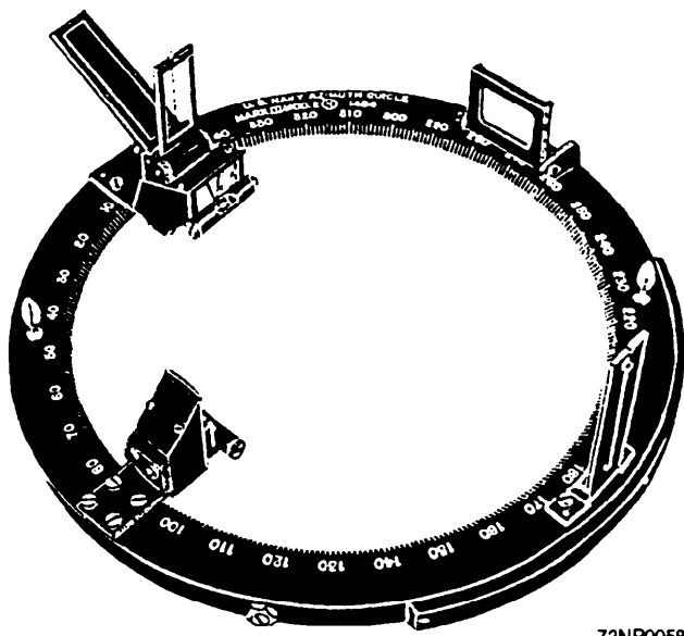
Figure 9-1.—Azimuth circle.
