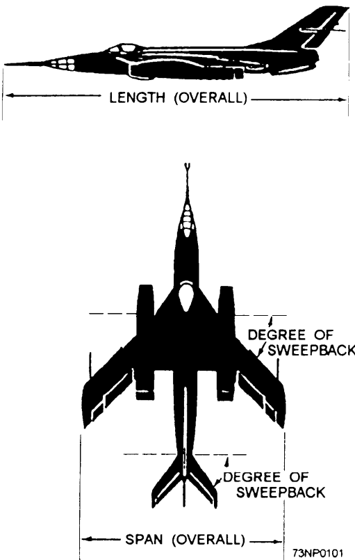
Figure 13-3.—Aircraft measurements.
