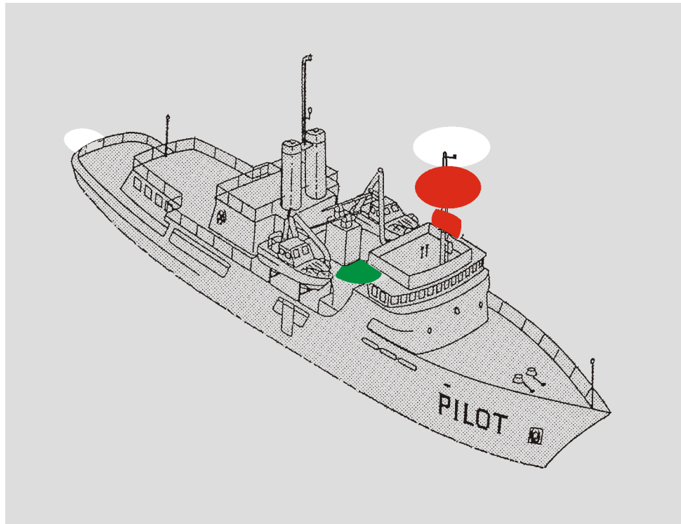
Figure 9-22.—Pilot vessel, under way.
